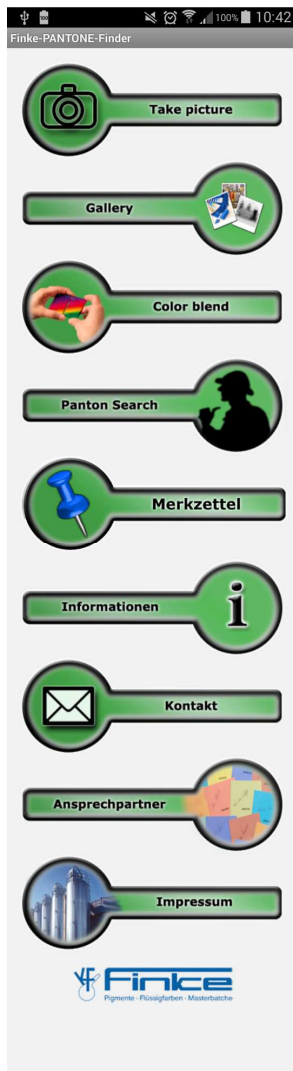
Finke-PAN-Finder-App Screenshot
